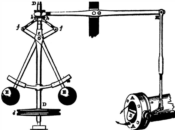
Figure 28.1 Watt’s centrifugal governor for a steam engine
